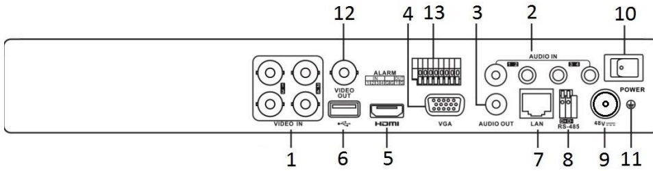
Figure 1-10 Rear Panel of DS-7200HUHI-K/P
