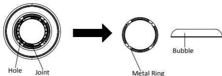
Figure 2-22 Remove the Metal Ring and the Bubble
