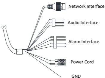
Figure 1-8 Cable Interfaces of Type IV Camera
