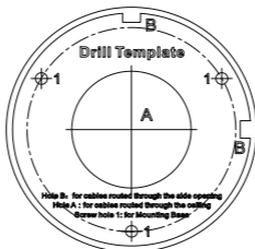
Figure 2-3 Drill Template for Junction Box
