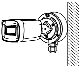
Figure 2-6 Fix the Junction Box Cover on Its Body
