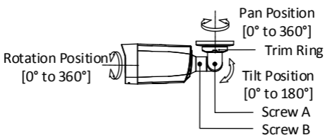
Figure 2-2 3-Axis Adjustment
